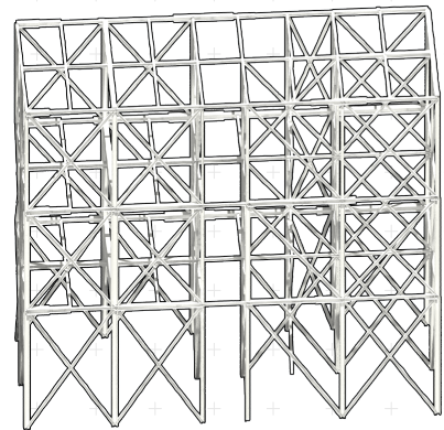
SECONDARY BUILDING CORE STRUCTURE
