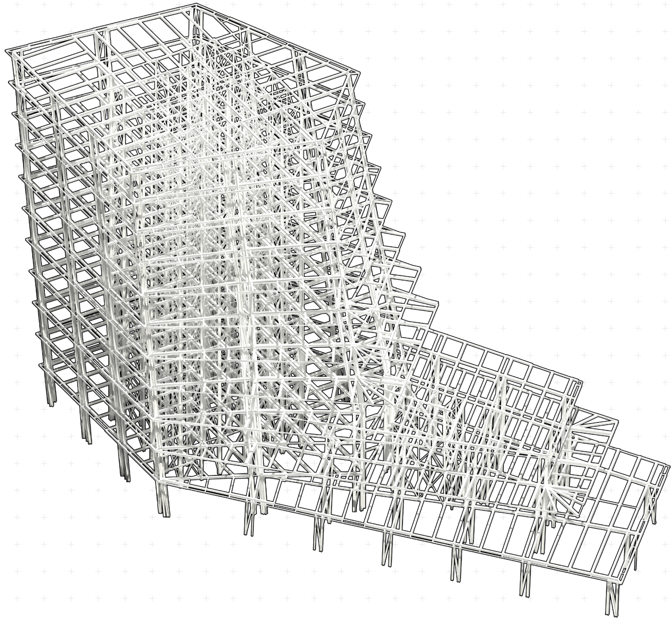
MAIN BUILDING STRUCTURE
