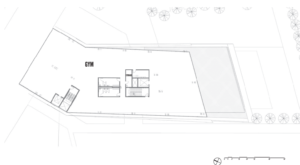
SECOND FLOOR - SECONDARY BUILDING
