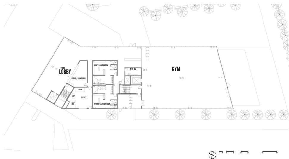
GROUND FLOOR - SECONDARY BUILDING
