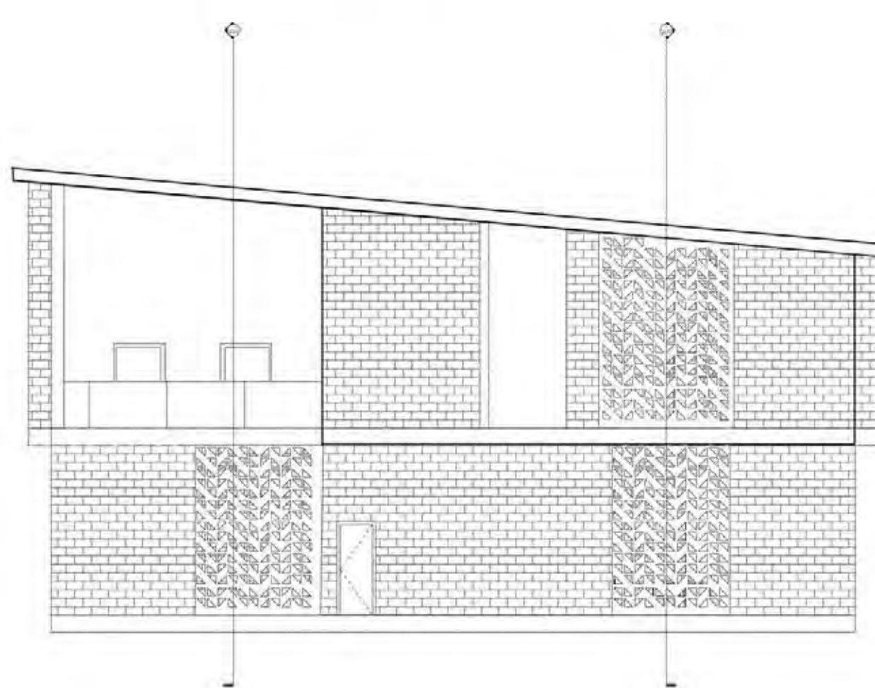
North Elevation and Section 1:100
