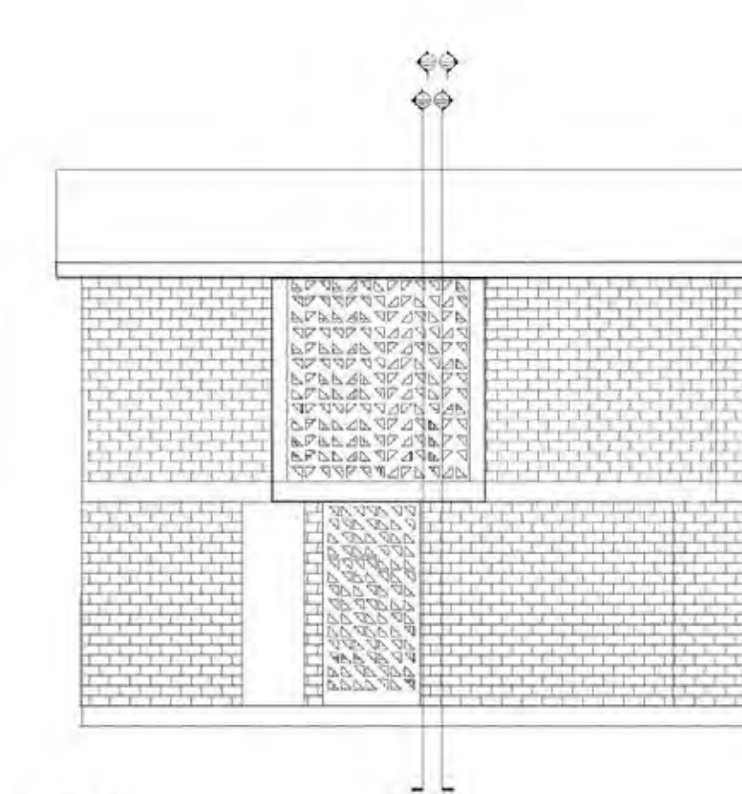
East Elevation and Section 1:100
