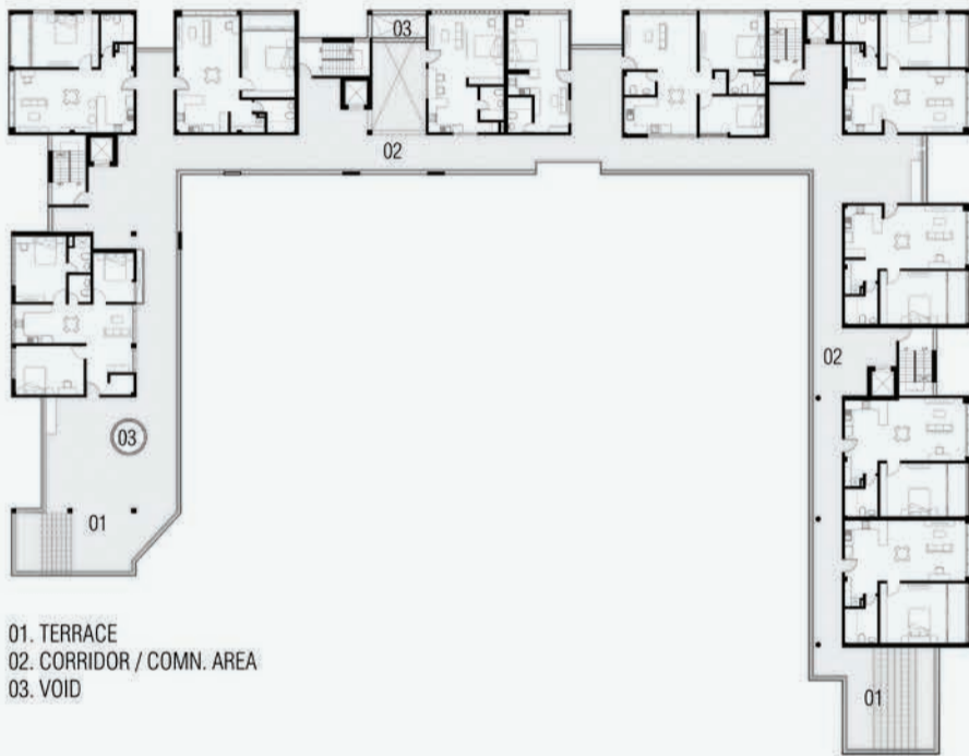
FORTH FLOOR Scale: 3/4" = 1'-00"
