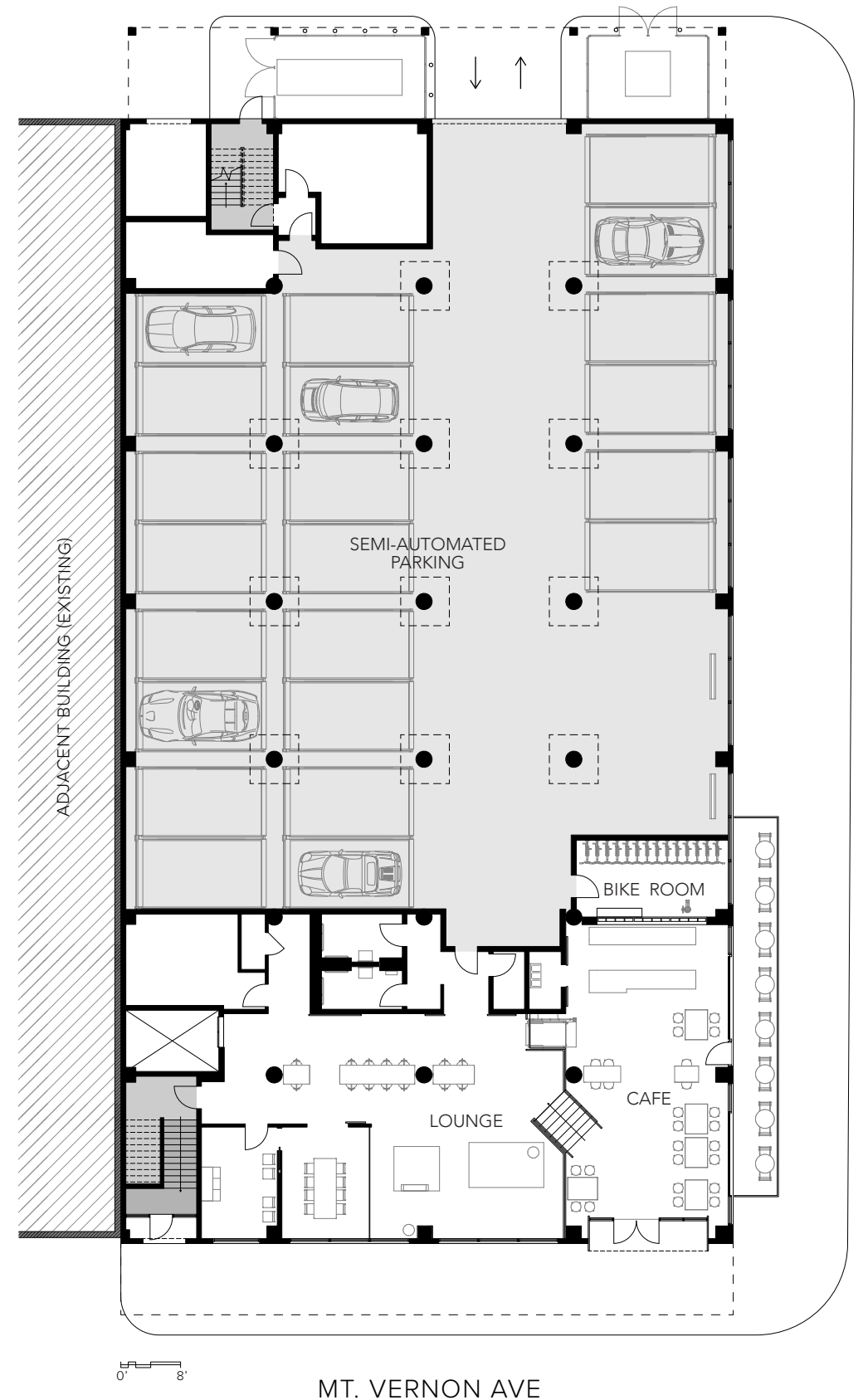
GROUND LEVEL & SITE PLAN WAREHOUSE
