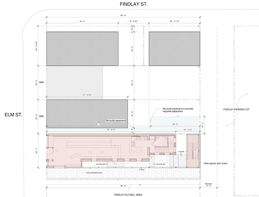
Site Plan
