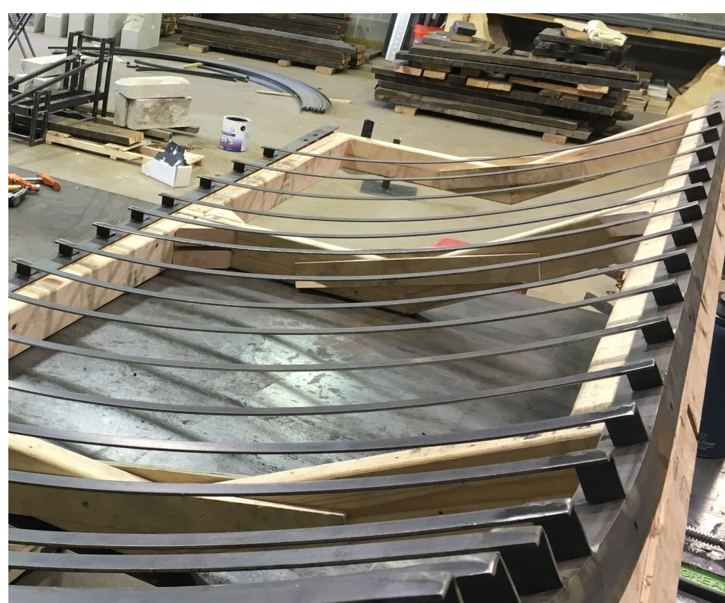
Steel angles and bars were bent on a roller and laid out on a custom jig to facilitate the precision welding of each frame.
