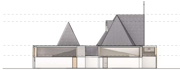
NORTH ELEVATION
